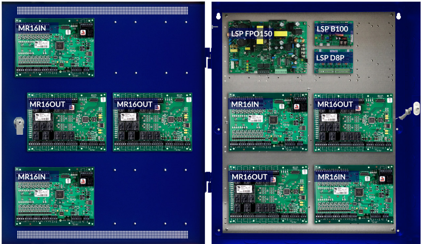
Diagram shows 1 of 2 enclosures with the same board layout
